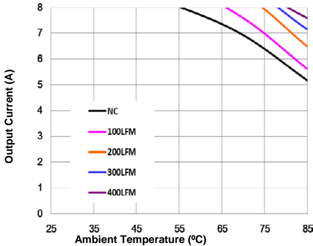
Figure 9. Current Derating Curve with Open Frame
