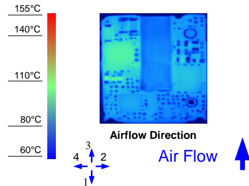
Figure 10. Thermal Image for Airflow Direction 3 (8A output, 55°C ambient, 200 LFM, typical V_{in} , open frame unit)
