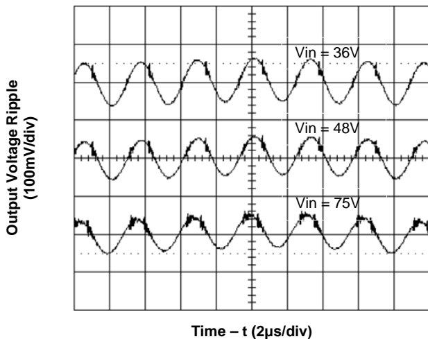
Figure 5. Output Ripple Voltage at Full Load (tested with 8x47µF ceramic output capacitors)
